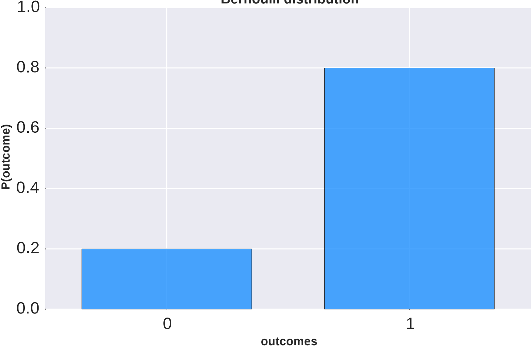
Bernoulli distribution
