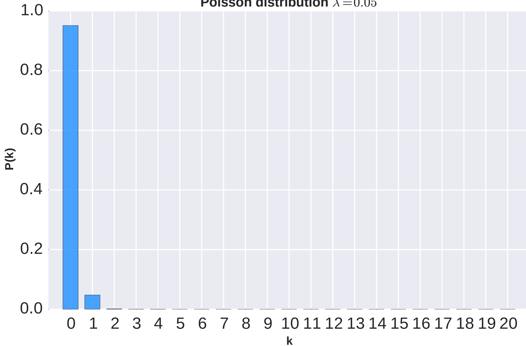
Poisson distribution \lambda=0.05
