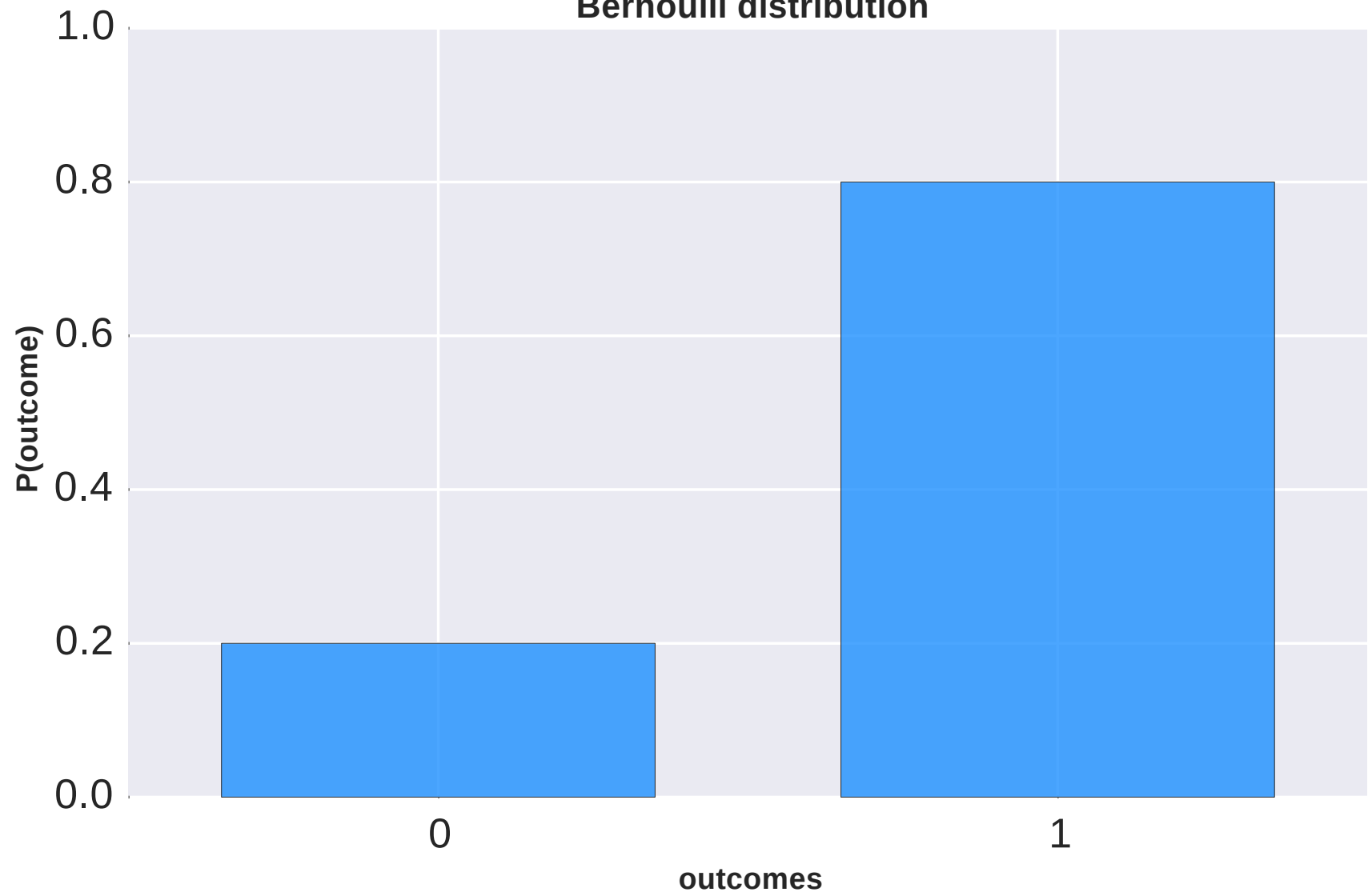
Bernoulli distribution
