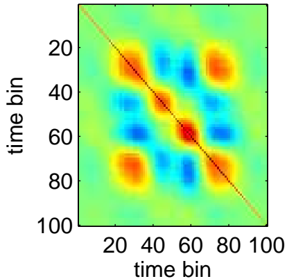
covariance matrix
