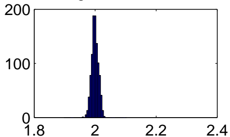
estimated slope sigma=1, n=1000
