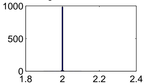
estimated slope sigma=1, n=1000
