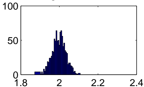
estimated slope sigma=1, n=100
