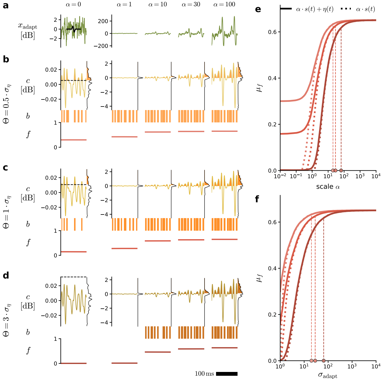
Fig. 6: Intensity invariance by thresholding and temporal averaging depends on both the threshold value and the noise floor. Synthetic input x_{\text{adapt}}(t) consists of song component s(t) scaled by \alpha with additive noise component \eta(t) . Input x_{\text{adapt}}(t) is transformed into kernel response c_i(t) , binary response b_i(t) , and feature f_i(t) . Threshold value \Theta_i is set to multiples of the reference standard deviation \sigma_\eta of c_i(t) for input x_{\text{adapt}}(t) = \eta(t) . Darker colors correspond to higher \Theta_i . Left: x_{\text{adapt}}(t) , c_i(t) , b_i(t) , and f_i(t) for different scales \alpha and threshold values \Theta_i . Left-most column is the pure-noise reference. Right: Average value of f_i(t) during the song for the different \Theta_i . a: Input x_{\text{adapt}}(t) . b-d: c_i(t) , b_i(t) , and f_i(t) for the different \Theta_i based on the same x_{\text{adapt}}(t) from a . e: Average value of f_i(t) during the song for the different \Theta_i in b-d .
