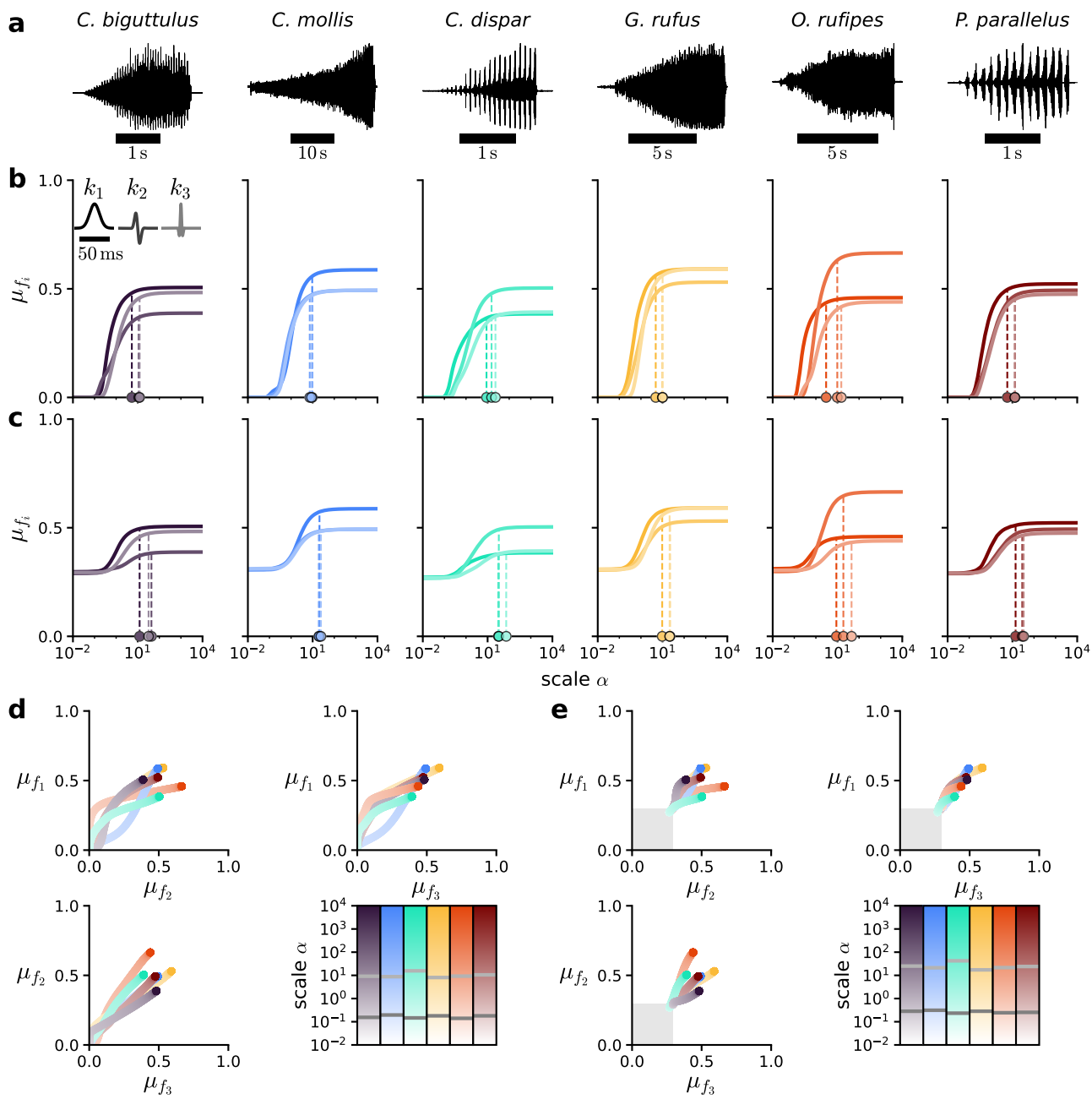
Fig. 7: Feature representation of different species-specific songs saturates at different points in feature space.
