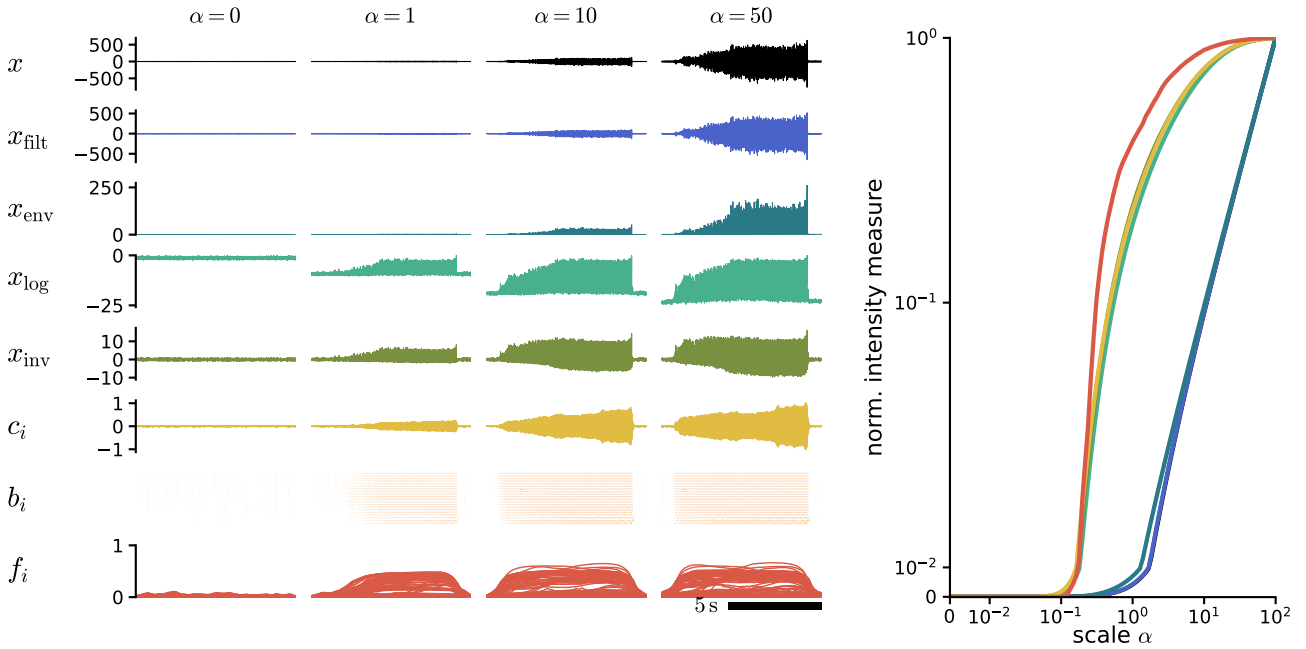
Fig. 8: Step-wise emergence of intensity invariant song representation along the model pathway.
