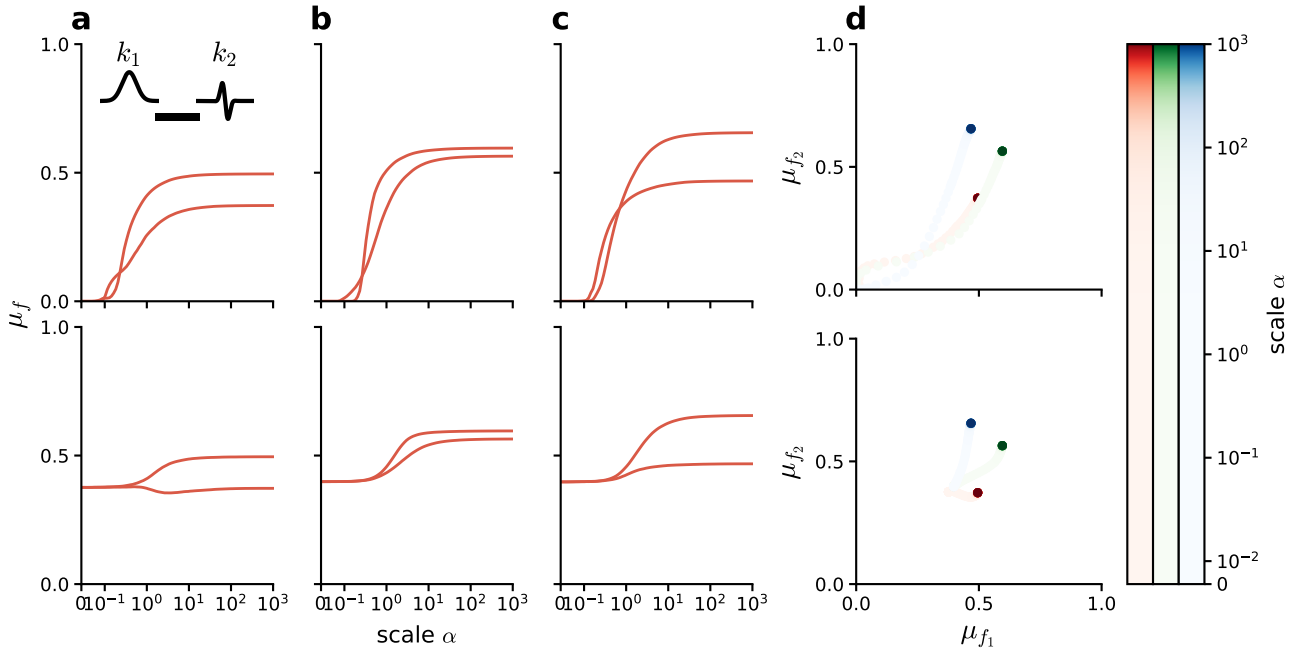
Fig. 7: Feature representation of different species-specific songs saturates at different points in feature space.
