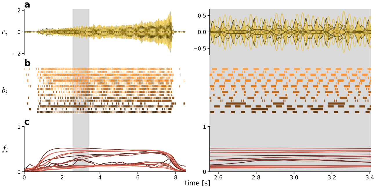
Fig. 3: Representations of a song of O. rufipes during the feature extraction stage. Different colors indicate Gabor kernels with different lobe number n and sign, with lighter colors for higher n ( 1 \leq n \leq 4 ; both + and - per n ; two kernel widths \sigma of 4 ms and 32 ms per sign). a: Kernel-specific filter responses. b: Binary responses. c: Finalized features.
