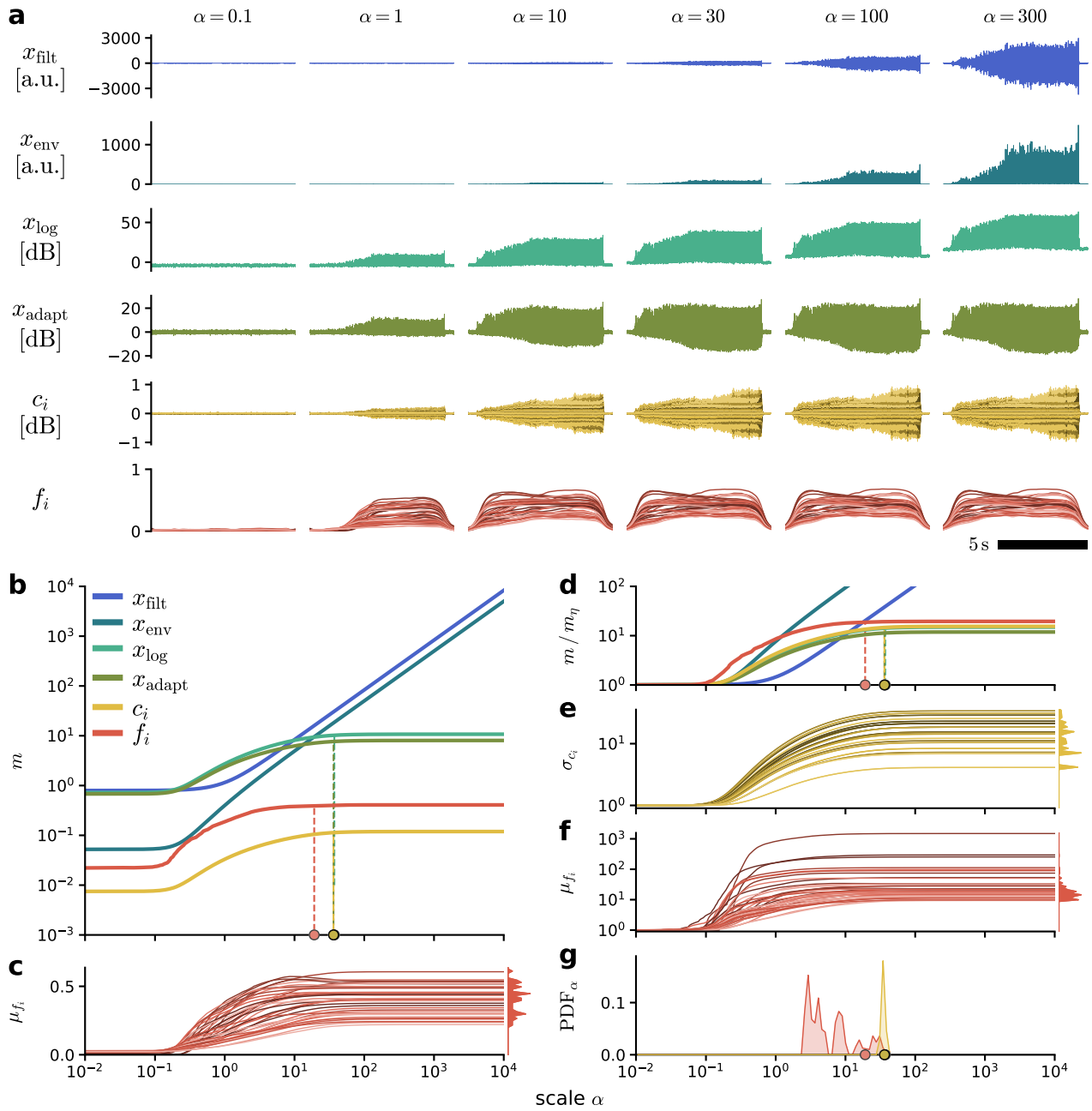
Fig. 8: Step-wise emergence of intensity invariant song representation along the model pathway.
