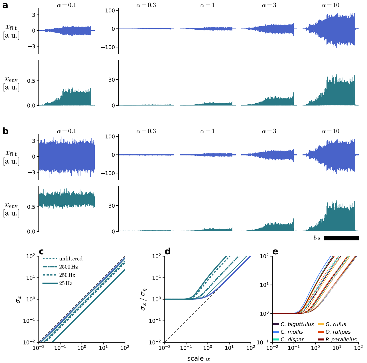
Fig. 4: Rectification and lowpass filtering improves SNR but does not contribute to intensity invariance. Input x_{\text{raw}}(t) consists of song component s(t) scaled by \alpha with optional noise component \eta(t) and is successively transformed into tympanal signal x_{\text{filt}}(t) and envelope x_{\text{env}}(t) . Different line styles indicate different cutoff frequencies f_{\text{cut}} of the lowpass filter extracting x_{\text{env}}(t) . Top: Example representations of x_{\text{filt}}(t) and x_{\text{env}}(t) for different \alpha . a: Noiseless case. b: Noisy case. Bottom: Intensity metrics over a range of \alpha . c: Noiseless case: Standard deviations \sigma_x of x_{\text{filt}}(t) and x_{\text{env}}(t) . d: Noisy case: Ratios of \sigma_x of x_{\text{filt}}(t) and x_{\text{env}}(t) to the respective reference standard deviation \sigma_\eta for input x_{\text{raw}}(t) = \eta(t) . e: Ratios of \sigma_x to \sigma_\eta of x_{\text{env}}(t) as in d for different species (averaged over songs and recordings, see appendix Fig. 13).
