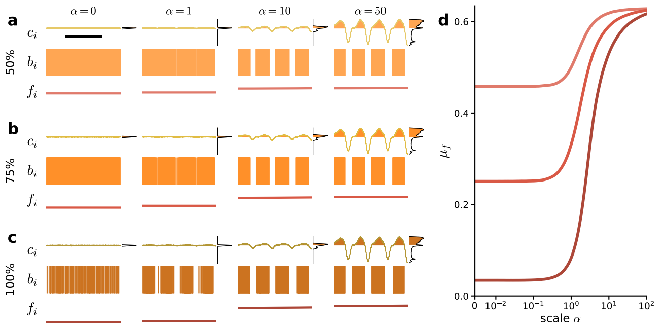
Fig. 6: Intensity invariance by thresholding and temporal averaging depends on noise. Kernel response c_i(t) is rescaled by \alpha , mixed with fixed-scale noise component \eta(t) , and transformed into binary response b_i(t) and further into feature f_i(t) . Threshold value \Theta_i is set to different percentiles of the the distribution of c_i(t) at \alpha = 1 . Darker colors indicate higher values of \Theta_i . Indicated time scale of 500 ms is the same for a-c (black bar). a : 50th percentile. b : 75th percentile. c : 100th percentile. d : Average value of f_i(t) during the song for the different \Theta_i in a-c .
