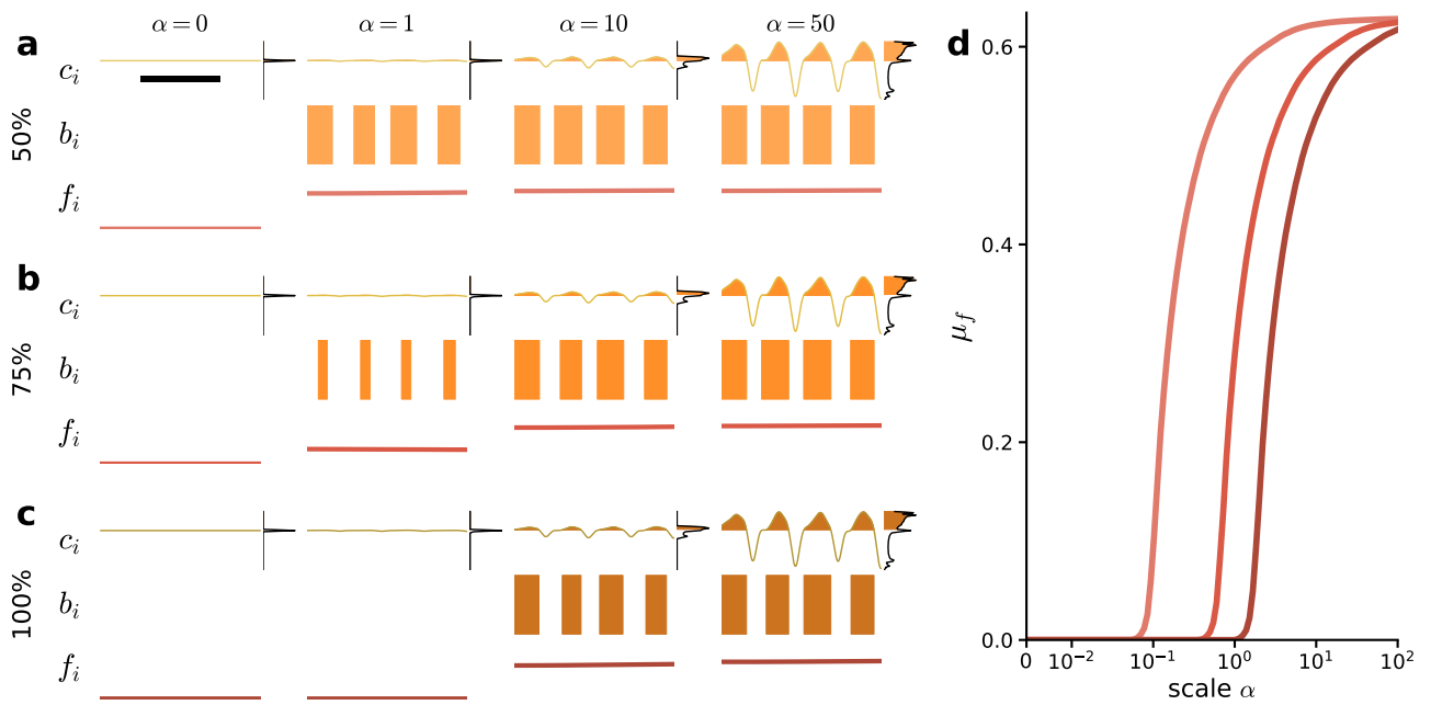
Fig. 5: Intensity invariance by thresholding and temporal averaging depends on the threshold value. Kernel response c_i(t) is rescaled by \alpha and transformed into binary response b_i(t) and further into feature f_i(t) . Threshold value \Theta_i is set to different percentiles of the the distribution of c_i(t) at \alpha = 1 . Darker colors indicate higher values of \Theta_i . Indicated time scale of 500 ms is the same for a-c (black bar). a: 50th percentile. b: 75th percentile. c: 100th percentile. d: Average value of f_i(t) during the song for the different \Theta_i in a-c.
