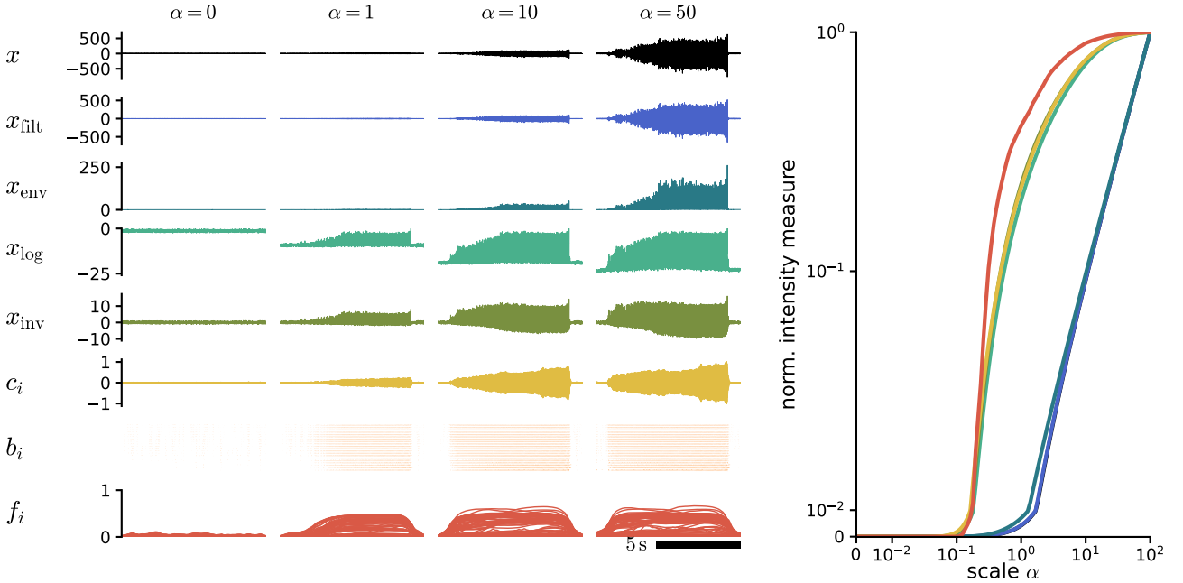
Fig. 7: Step-wise emergence of intensity invariant song representation along the model pathway.
