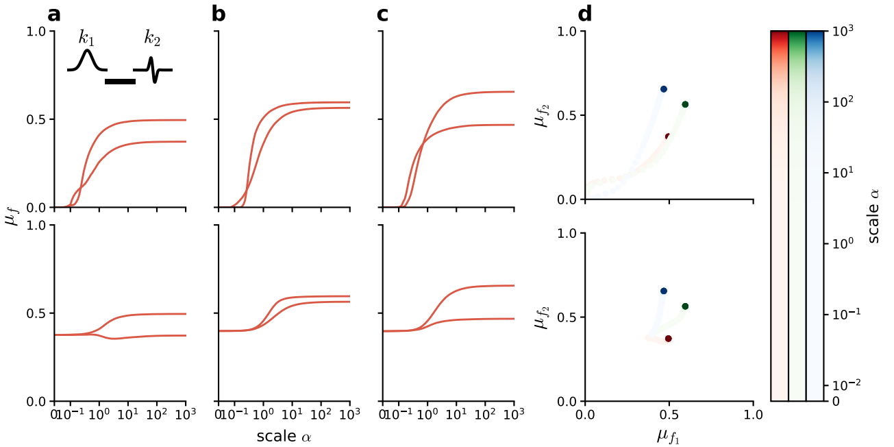
Fig. 6: Feature representation of different species-specific songs saturates at different points in feature space.
