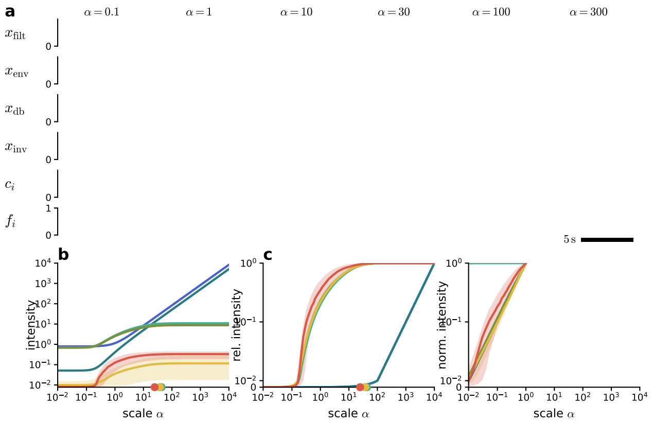
Fig. 7: Step-wise emergence of intensity invariant song representation along the model pathway.
