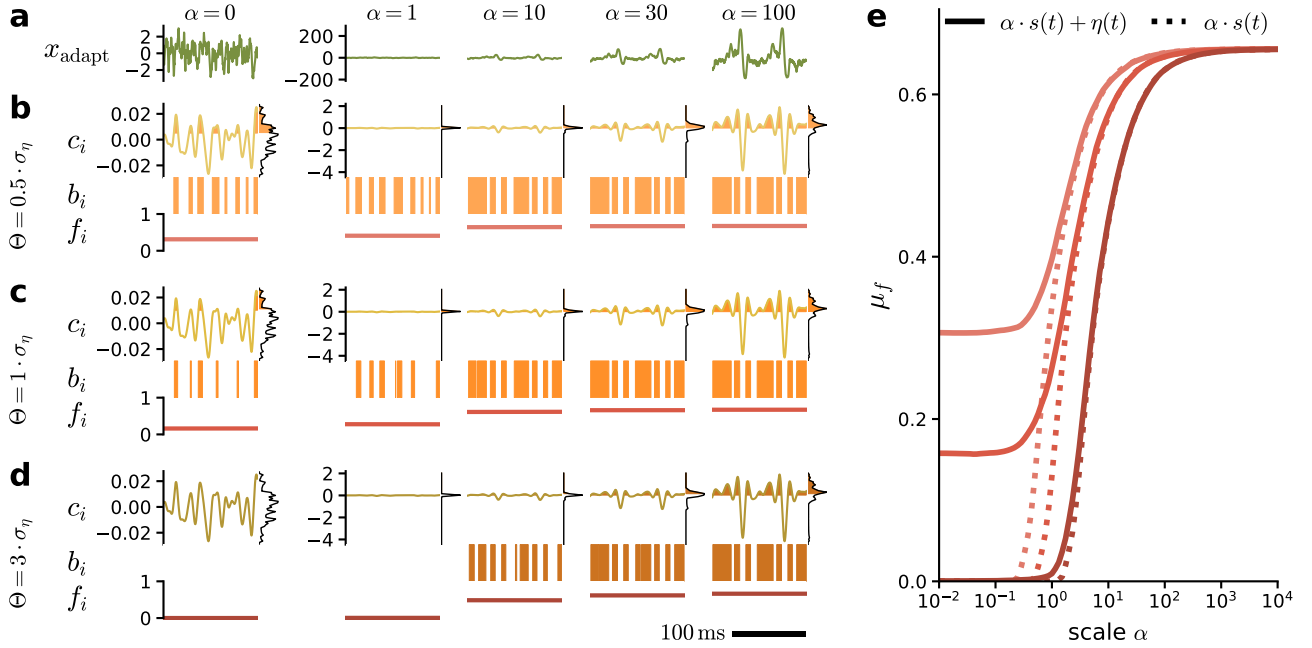
Fig. 5: Intensity invariance by thresholding and temporal averaging depends on both the threshold value and the noise floor. Synthetic input x_{\text{adapt}}(t) consists of song component s(t) scaled by \alpha with additive noise component \eta(t) . Input x_{\text{adapt}}(t) is transformed into kernel response c_i(t) , binary response b_i(t) , and feature f_i(t) . Threshold value \Theta_i is set to multiples of the reference standard deviation \sigma_\eta of c_i(t) for input x_{\text{adapt}}(t) = \eta(t) . Darker colors correspond to higher \Theta_i . Left: x_{\text{adapt}}(t) , c_i(t) , b_i(t) , and f_i(t) for different scales \alpha and threshold values \Theta_i . Left-most column is the pure-noise reference. Right: Average value of f_i(t) during the song for the different \Theta_i . a: Input x_{\text{adapt}}(t) . b-d: c_i(t) , b_i(t) , and f_i(t) for the different \Theta_i based on the same x_{\text{adapt}}(t) from a . e: Average value of f_i(t) during the song for the different \Theta_i in b-d .
