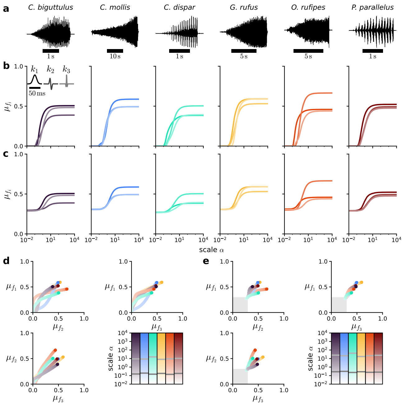
Fig. 6: Feature representation of different species-specific songs saturates at different points in feature space.
