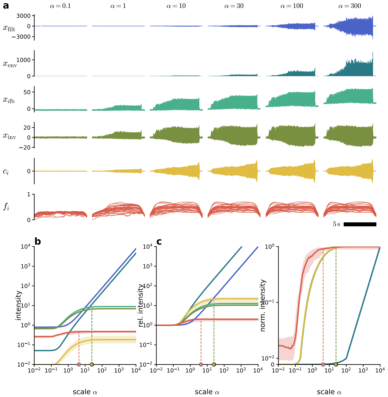
Fig. 7: Step-wise emergence of intensity invariant song representation along the model pathway.
