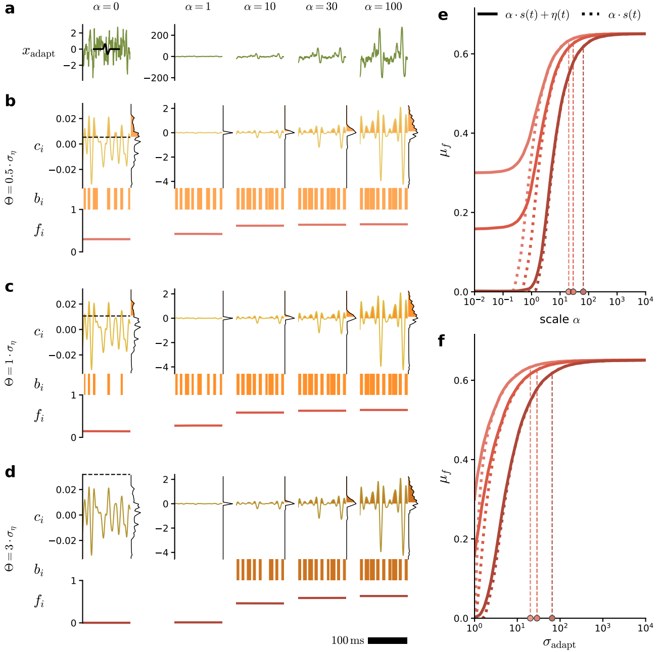
Fig. 5: Intensity invariance by thresholding and temporal averaging depends on both the threshold value and the noise floor. Synthetic input x_{\text{adapt}}(t) consists of song component s(t) scaled by \alpha with additive noise component \eta(t) . Input x_{\text{adapt}}(t) is transformed into kernel response c_i(t) , binary response b_i(t) , and feature f_i(t) . Threshold value \Theta_i is set to multiples of the reference standard deviation \sigma_\eta of c_i(t) for input x_{\text{adapt}}(t) = \eta(t) . Darker colors correspond to higher \Theta_i . Left: x_{\text{adapt}}(t) , c_i(t) , b_i(t) , and f_i(t) for different scales \alpha and threshold values \Theta_i . Left-most column is the pure-noise reference. Right: Average value of f_i(t) during the song for the different \Theta_i . a: Input x_{\text{adapt}}(t) . b-d: c_i(t) , b_i(t) , and f_i(t) for the different \Theta_i based on the same x_{\text{adapt}}(t) from a . e: Average value of f_i(t) during the song for the different \Theta_i in b-d .
