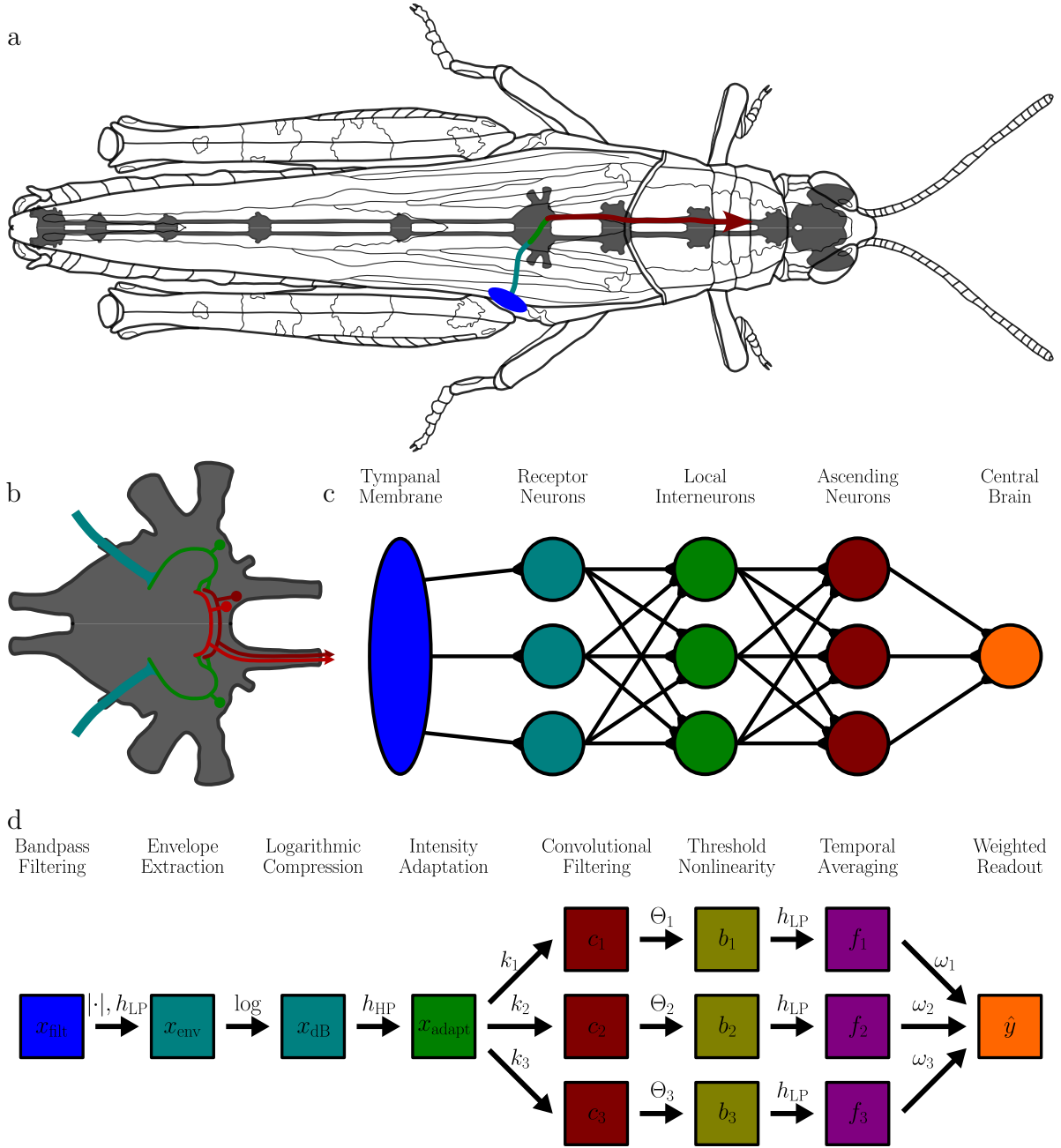
Figure 1: The auditory system of grasshoppers.
