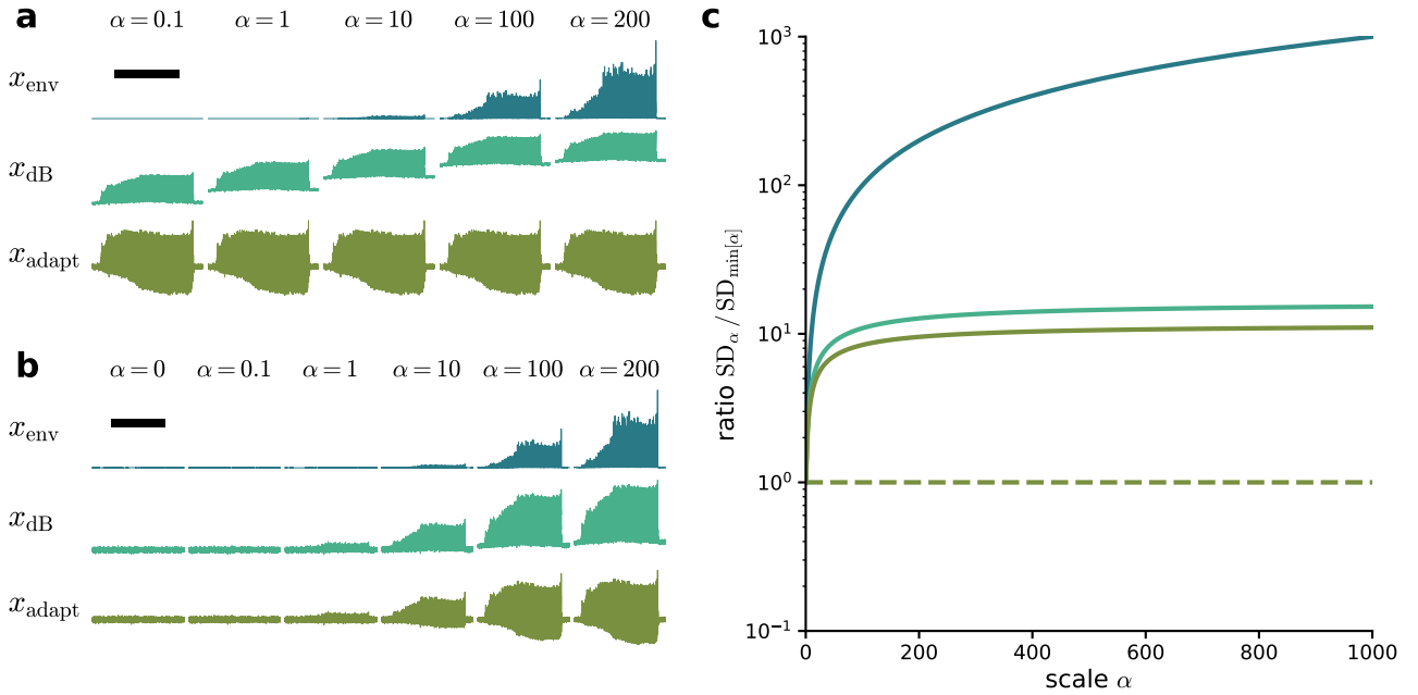
Fig. 4: Intensity invariance by logarithmic compression and adaptation is restricted by the noise floor. Synthetic envelope x_{\text{env}}(t) is transformed into logarithmically compressed envelope x_{\text{dB}}(t) and further into intensity-adapted envelope x_{\text{adapt}}(t) . Indicated time scale is 5 s for both a and b (black bars). a : Ideally, if x_{\text{env}}(t) consists only of song component s(t) rescaled by \alpha , then x_{\text{adapt}}(t) is fully intensity-invariant across all \alpha . b : In practice, x_{\text{env}}(t) also contains fixed-scale noise component \eta(t) , which limits the effective intensity invariance of x_{\text{adapt}}(t) to sufficiently large \alpha . c : Ratios of the SD of each representation in b at a given \alpha relative to the SD of the representation for \alpha = 0 (solid lines). The same ratios for the ideal x_{\text{adapt}}(t) in a are shown for comparison (dashed line).
