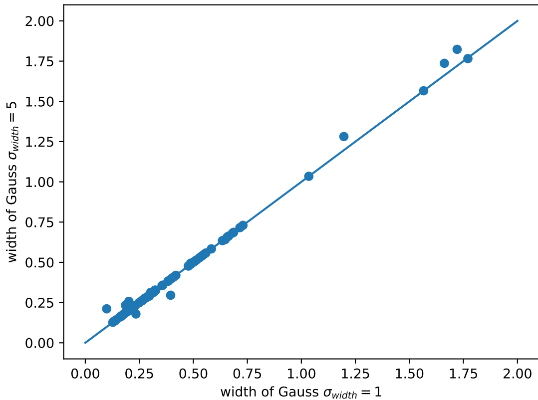
100 bins
