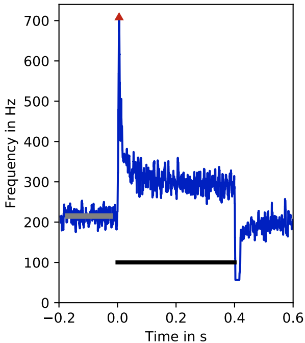
Step Response
