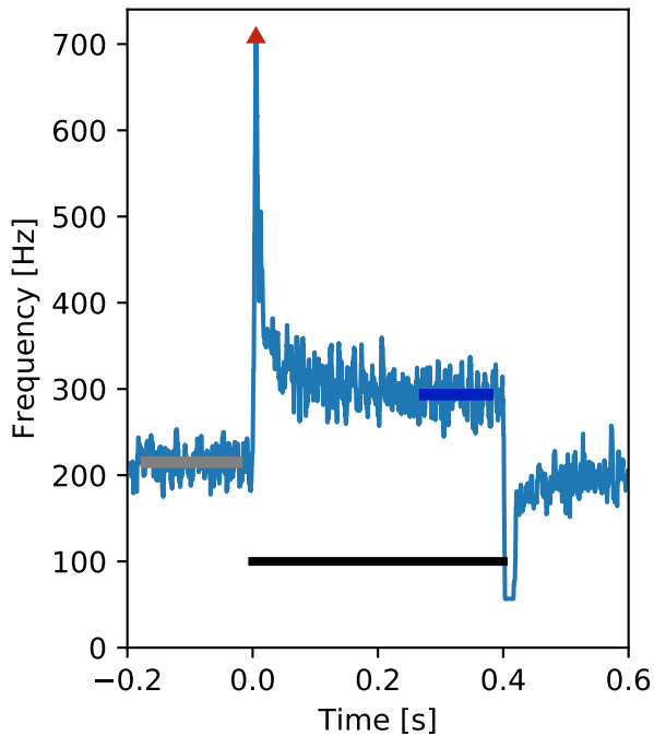
Step Response
