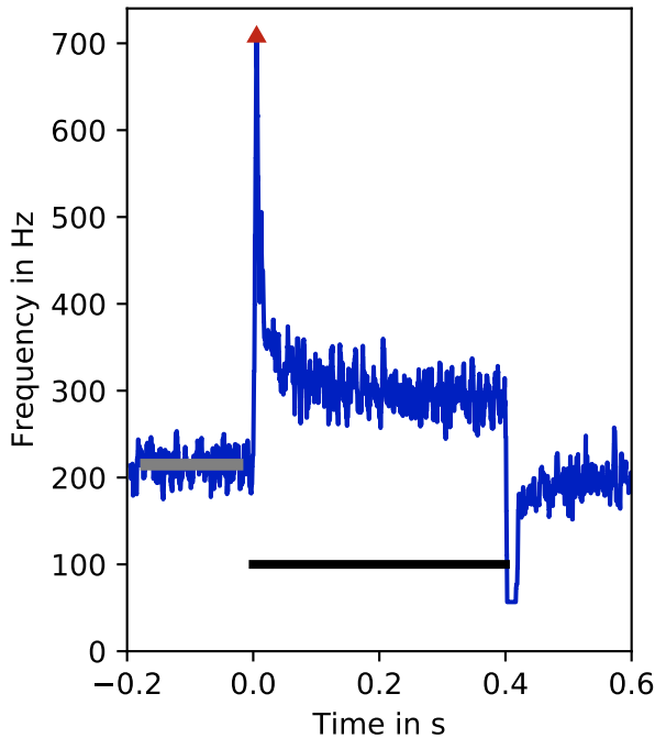
Step Response
